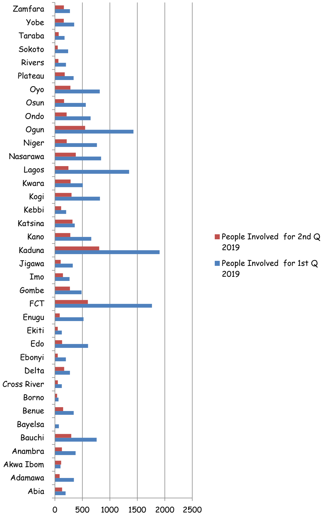
Chart 21: People Involved on State Basis
