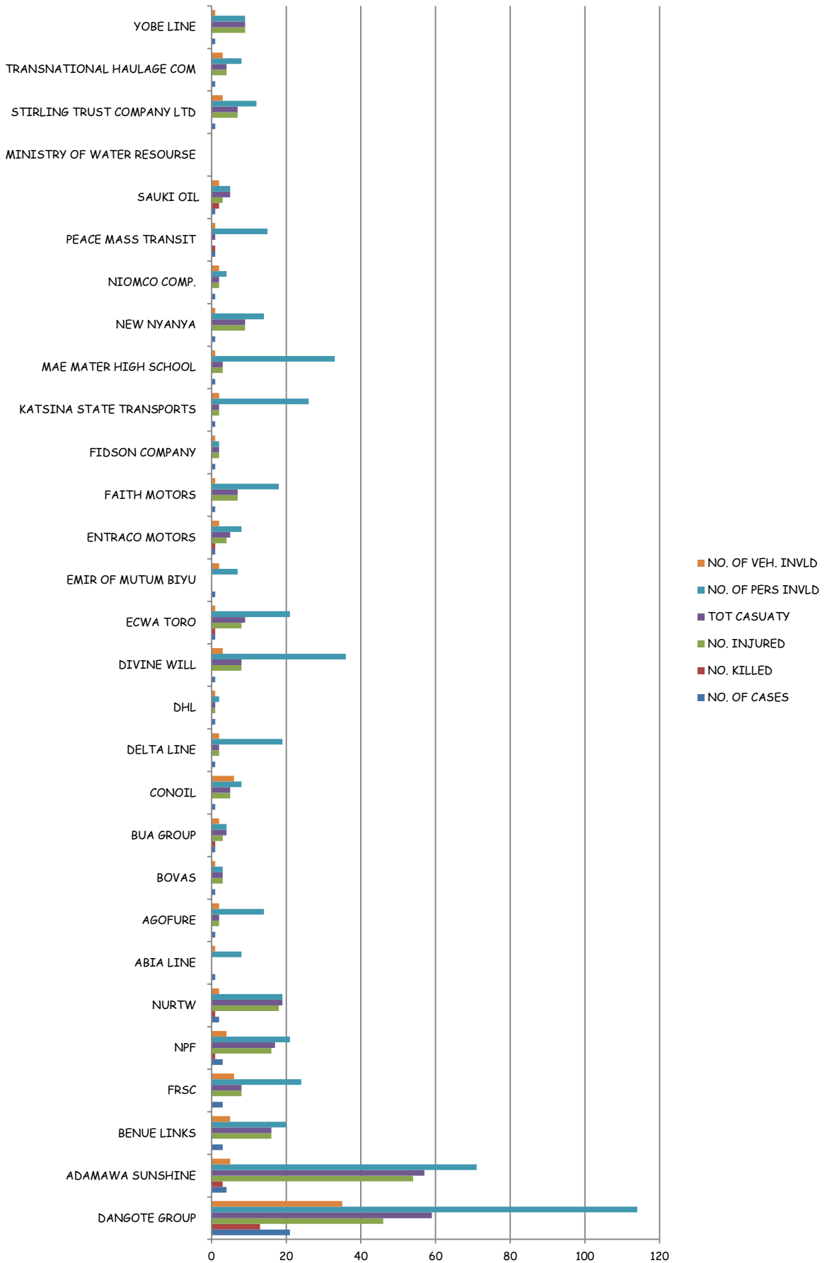
Chart 14: Summary Of RTC Involving Fleet Operators
