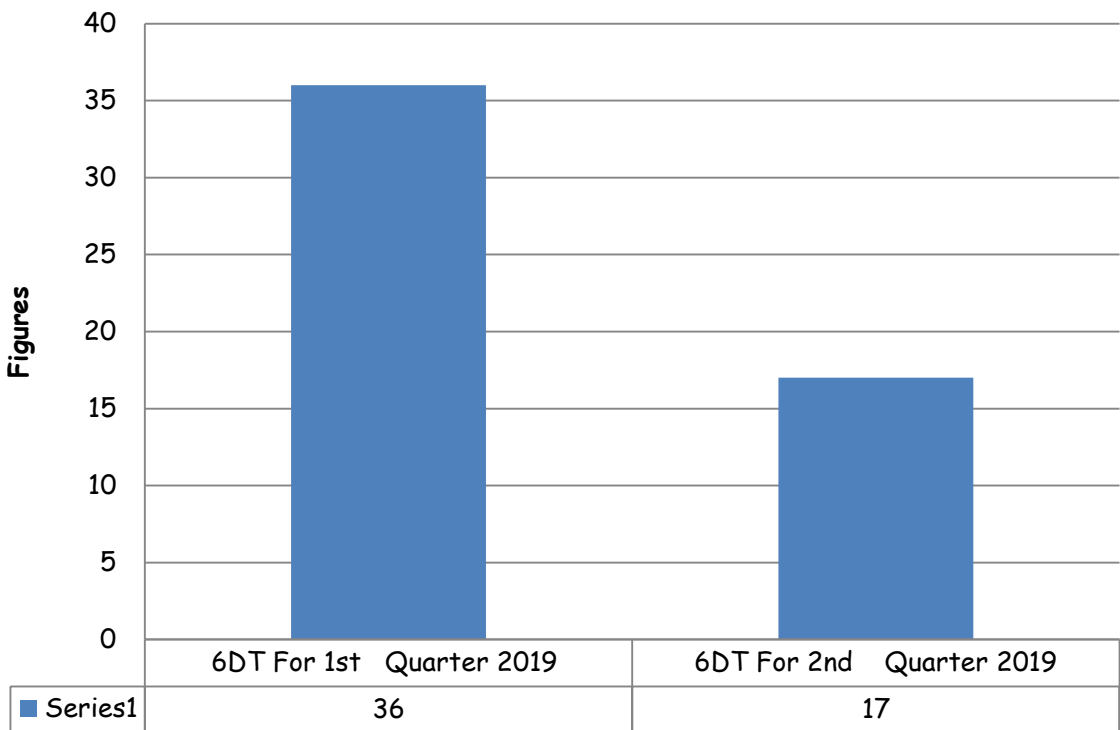
Chart 24: 6DT Accident Investigated For 1st Q 2019 and 2nd Q 2019
