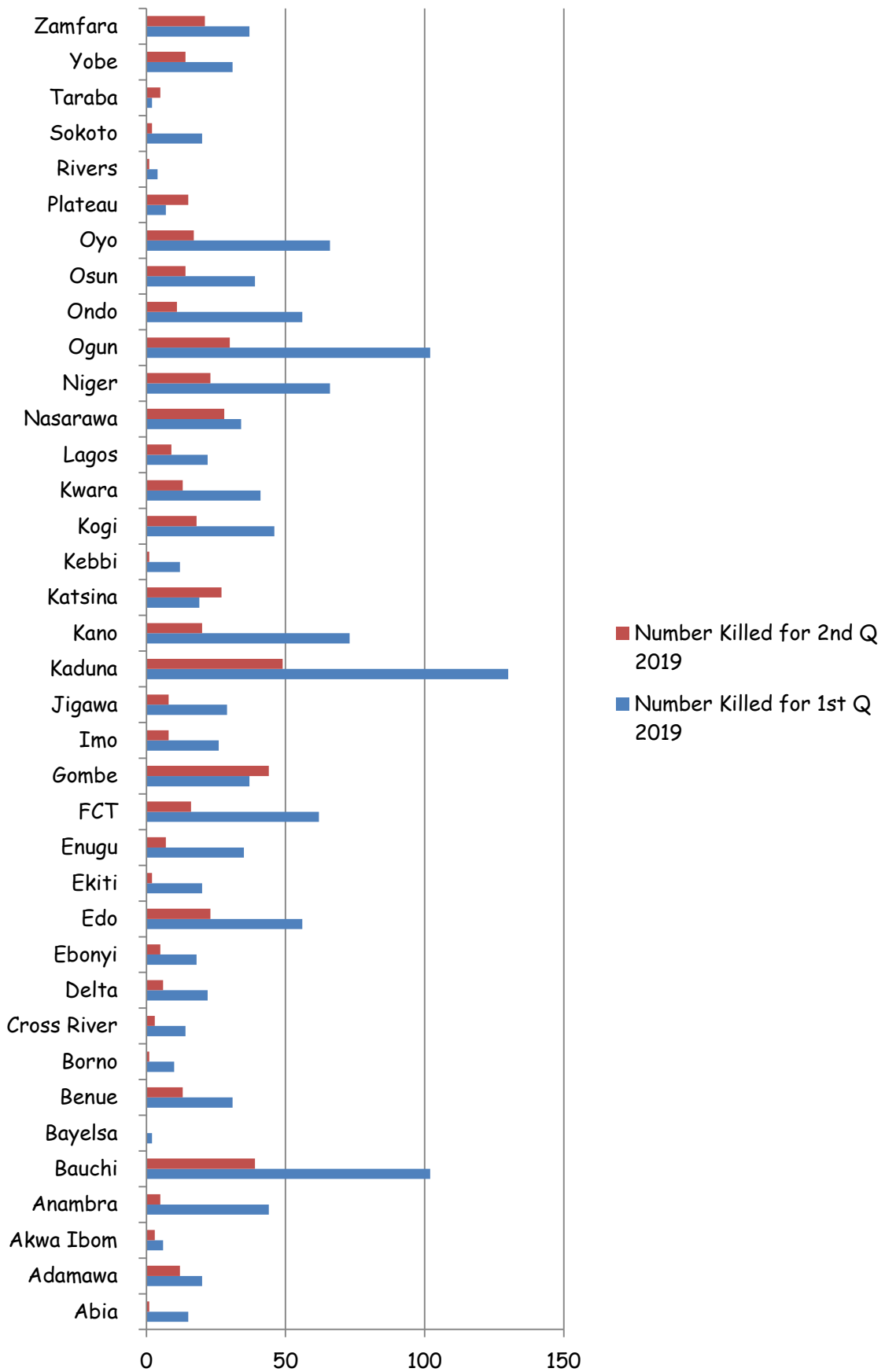
Chart 20: Number Killed on State Basis
